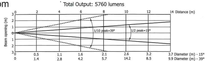
LEDWash600X Photometrics
