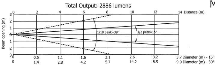
LEDWash300X Photometrics
